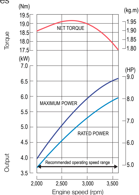
Power Curves
